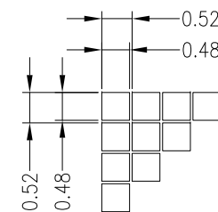
DETAIL A (SCALE 10:1)
